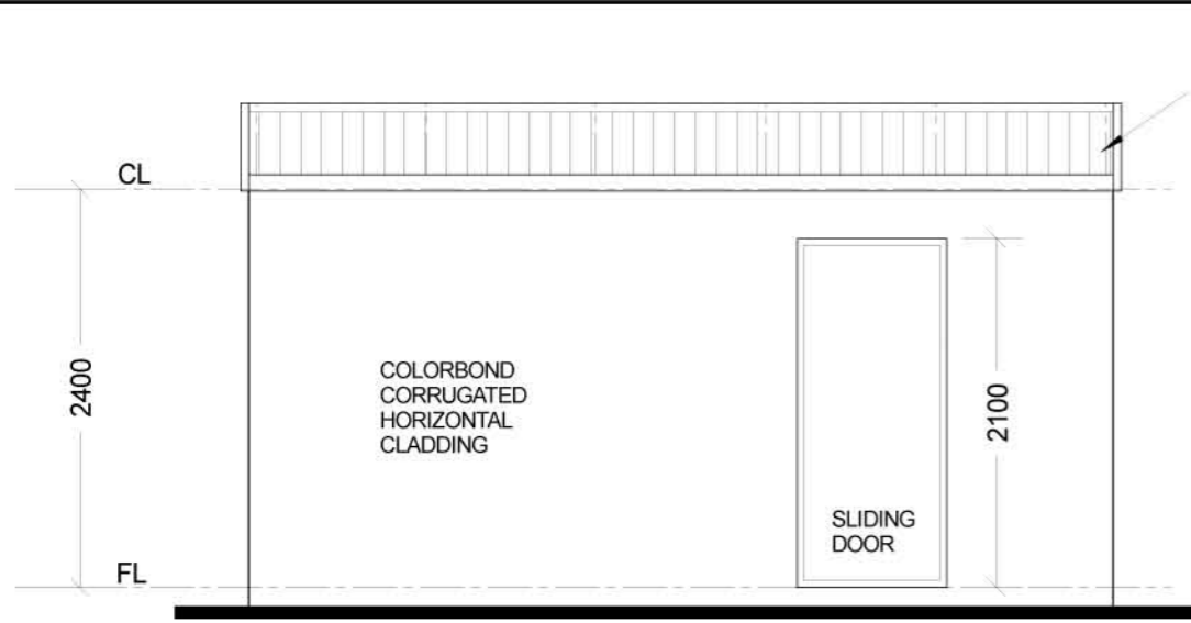
ELEVATION 1 SCALE 1:50
