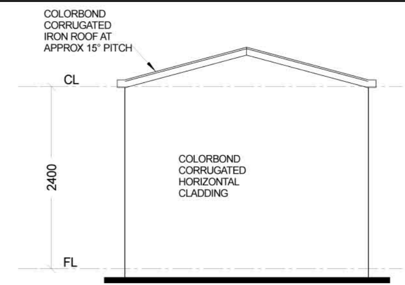
ELEVATION 3 SCALE 1:50
