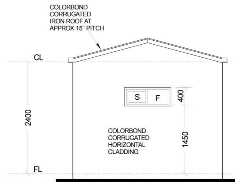
ELEVATION 4 SCALE 1:50
