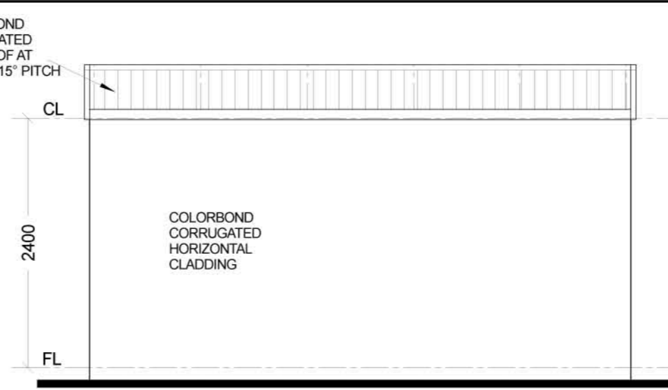
ELEVATION 2 SCALE 1:50
