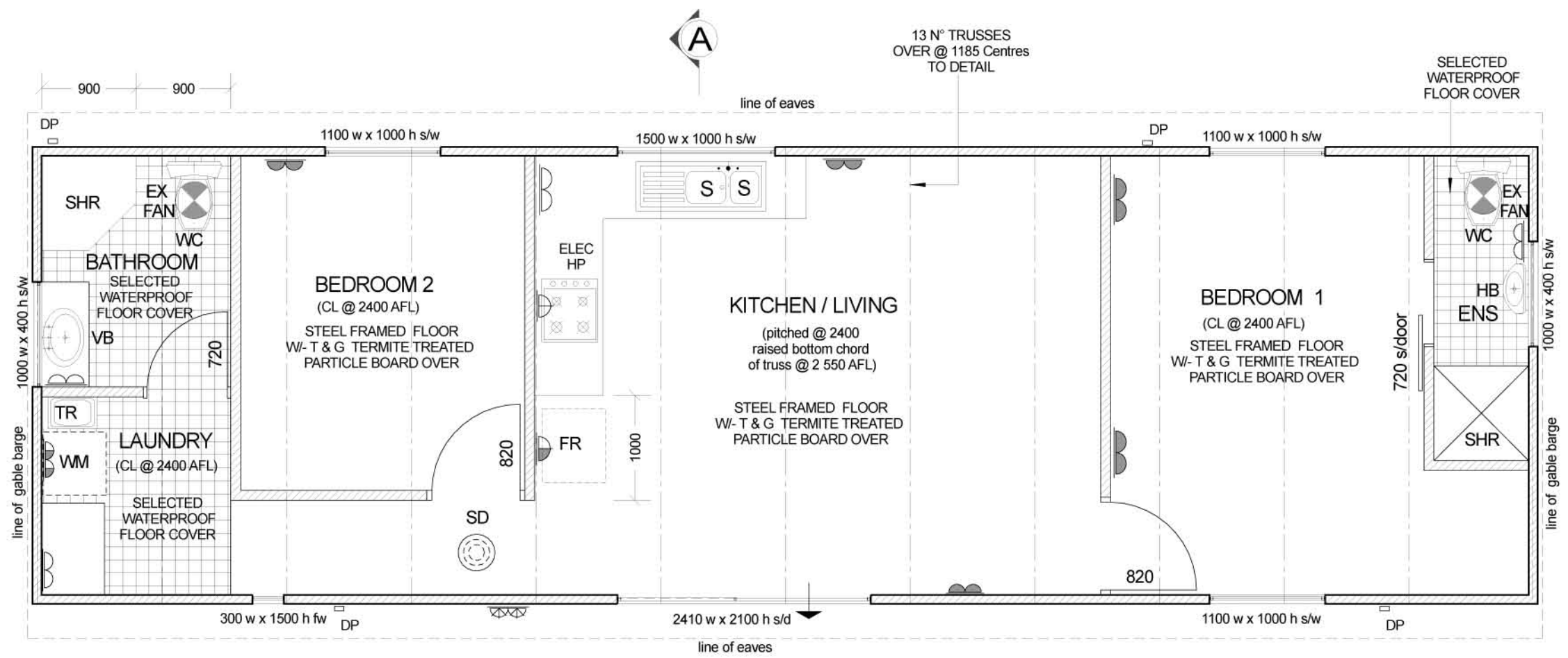
FLOOR PLAN scale 1:50
