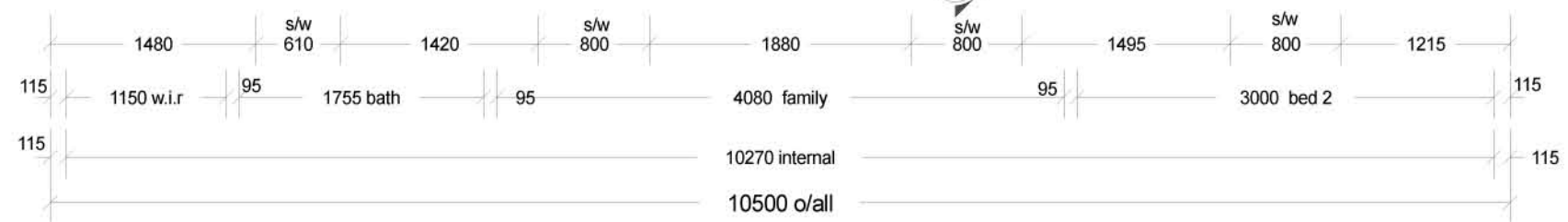
FLOOR PLAN scale 1:50
